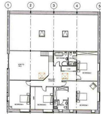
First Floor Plan 1:100
